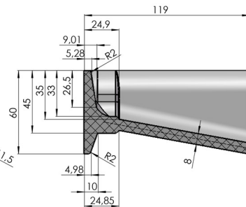
SECTION A SCALE 1 : 1.5
